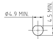
RECOMMENDED SMB MOUNTING HOLE
