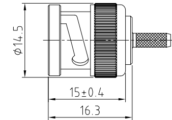
BNC DETAIL DRAWING
